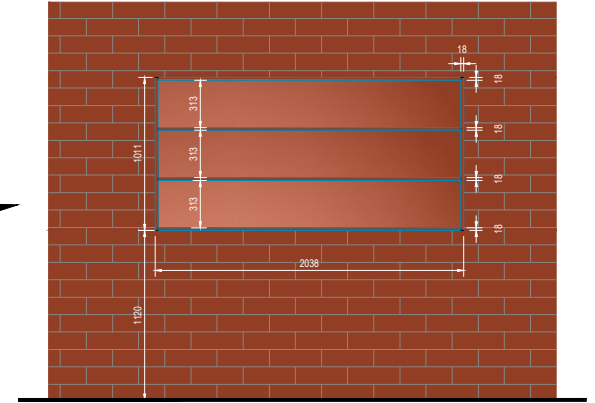
02 PROPOSED NICHE DETAIL Scale 1:50
